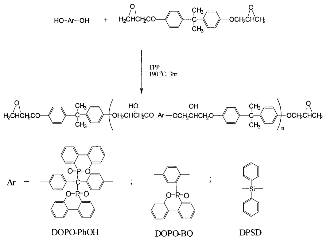
Scheme 2 Preparation of epoxies via the fusion process.
